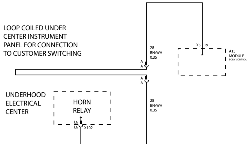
WIRING PROVISION FOR HORN-SIREN CIRCUIT OPTION 6J4
