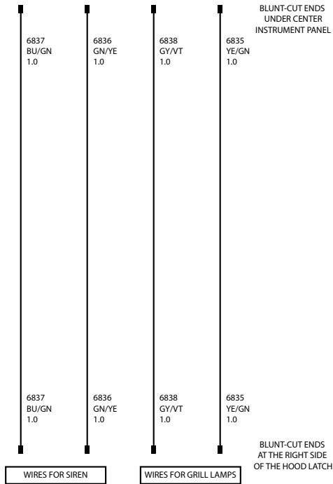
WIRING PROVISION FOR GRILLE LAMPS AND SPEAKER/SIREN OPTION 6J3
