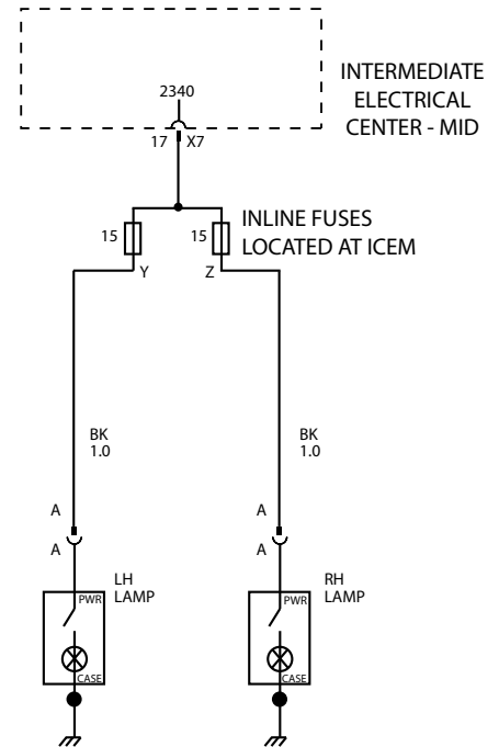
LAMP BULBS - HALOGEN H7635
